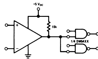
Figure 10. Driving TTL
