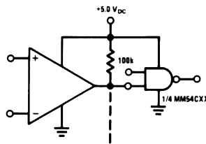
Figure 9. Driving CMOS
